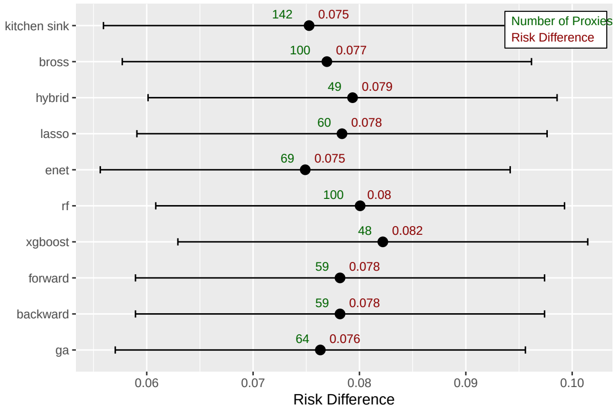
Risk Difference with 95% Confidence Intervals by Methods
